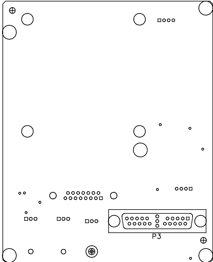
E1938-20007 REV C COMPONENT LOCATOR BOTTOMSIDE 05/21/97
